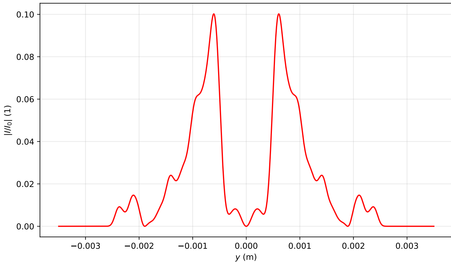
Intensity profile I(x=0, y, z=3.264)/I_0 , P_{in}=8.0P_{cr} , artificial time
